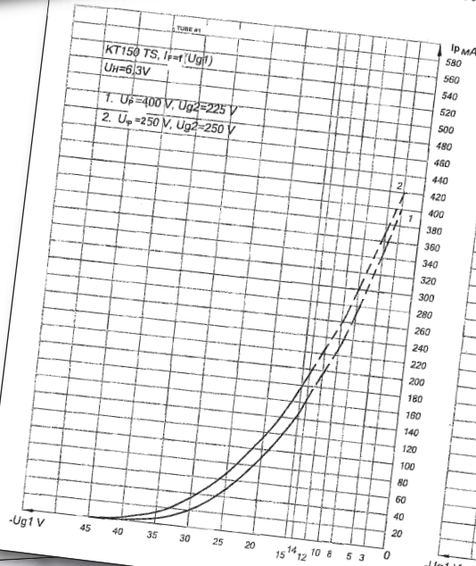
Grid-plate characteristics
