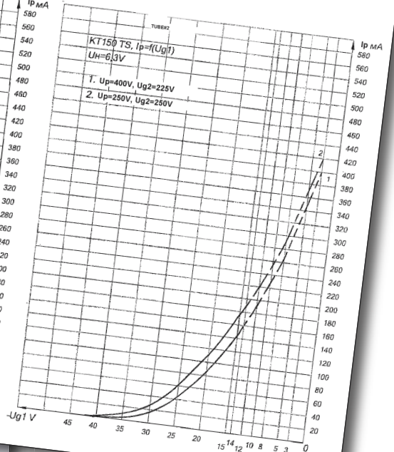
Grid-plate characteristics
