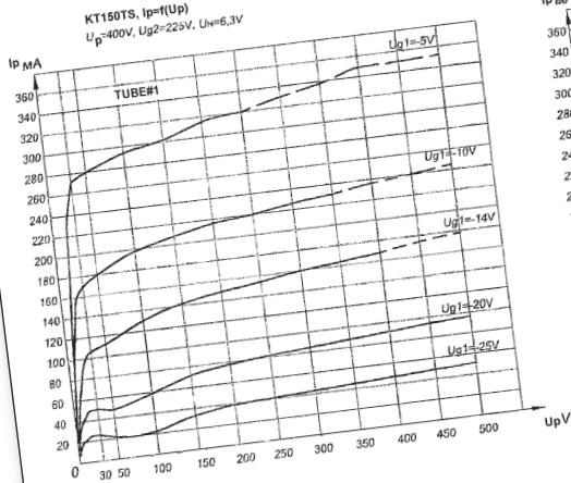
Plate characteristics
